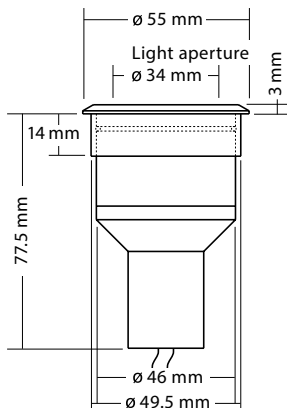
Halogen and HP LED technology round top plate with mounting sleeve
