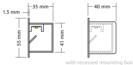
with recessed mounting box
