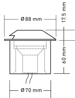
Standard HL-LED
