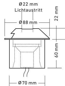
Plus HL-LED
