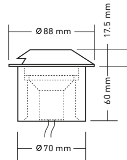
Standard HL-LED
